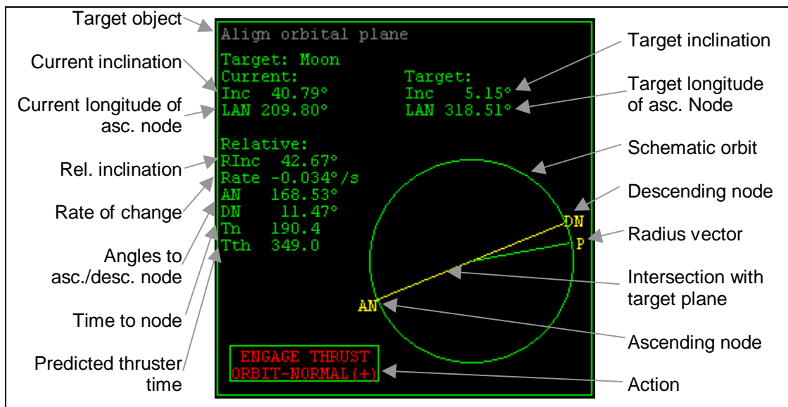
Figure 15: Align Orbital Plane MFD mode.
