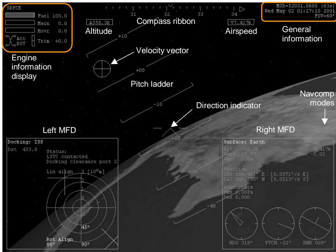
Figure 6: HUD in surface mode, including docking and surface MFDs.
