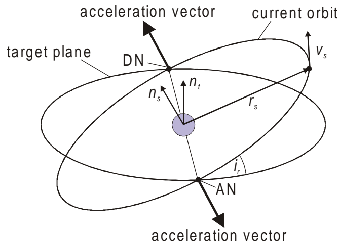
Figure 21: Alignment of the orbital plane. r_s : radius vector. v_s : velocity vector. AN: ascending node. DN: Descending node. n_s : normal of the current plane. n_t : normal of the target plane.
