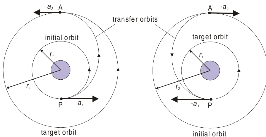
Figure 20: Moving into a higher orbit involves prograde acceleration at P and A (periapsis and apoapsis of the transfer orbit). Conversely, moving from the higher to the lower orbit requires retrograde acceleration at A and P.
