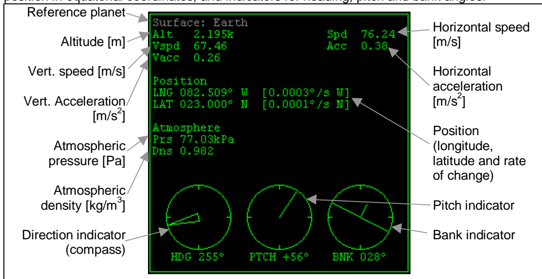
Figure 13: Surface MFD.
