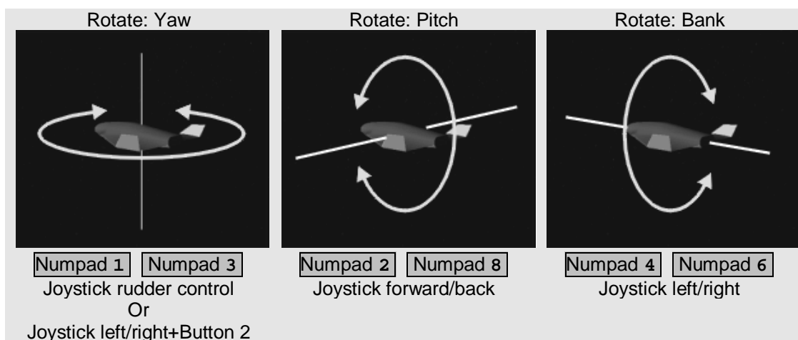
Figure 18: Attitude thrusters in rotational mode.
