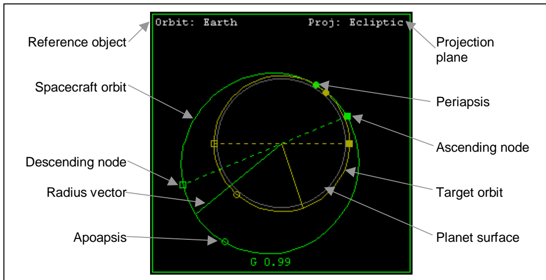
Figure 10: Orbit MFD in graphic mode.
