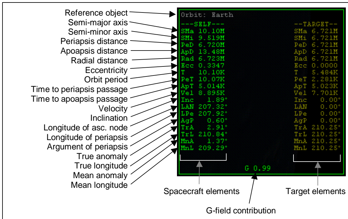
Figure 9: Orbit MFD in parameter list mode.
