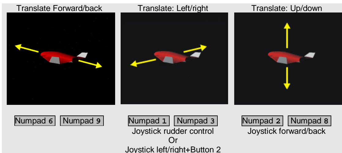
Figure 19: Attitude thrusters in translational (linear) mode.
