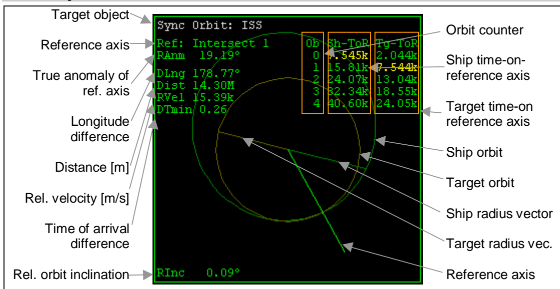
Figure 16: Synchronise Orbit MFD mode.
