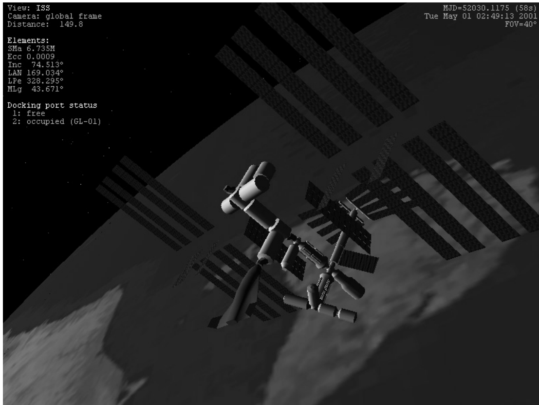
Figure 23: A successfully completed docking approach to the ISS.
