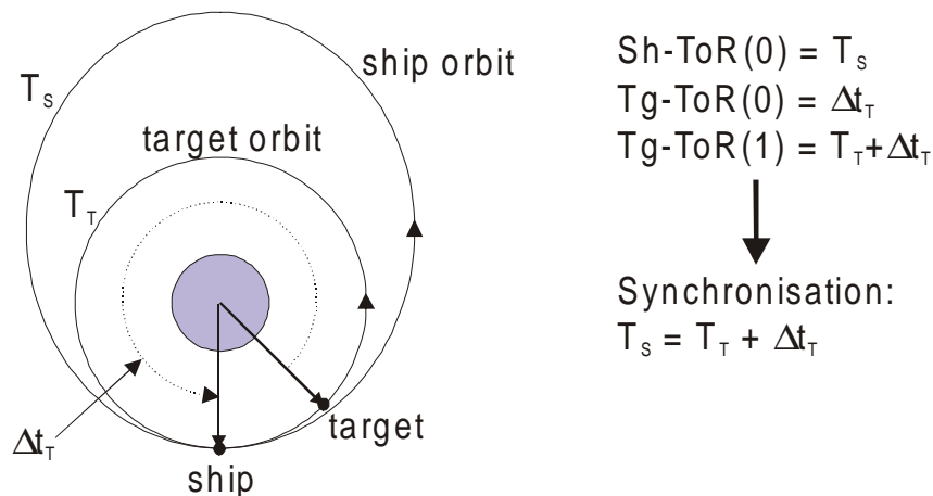
Figure 22: A transition orbit to intercept the target at the next periapsis passage.
